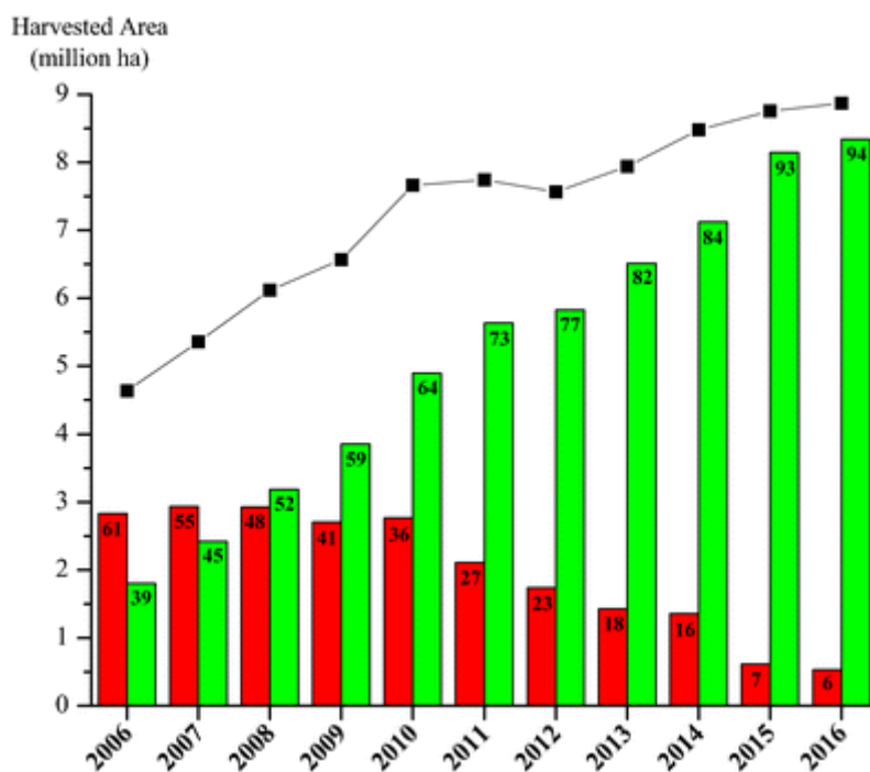
Figure 3 Total harvested area (black line) in south-central Brazil and evolution (in percentage) of the type of harvest during 2006–2016: manual burned (red bars) versus green mechanized (green bars)
