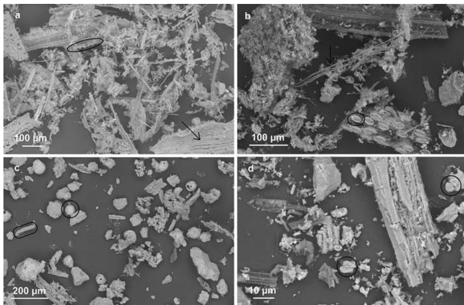
Figure 2 SEM (BSE) images of the ash samples a) silica trilobite phytoliths (circled) and elongated silica cells (arrow), (b) silica-edged stomata (circles) and carbonaceous fibre bundle (arrow), (c) spherical silicate and prismatic silica particles (circled) and d) two phytoliths bodies (circled)
